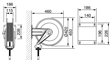
Series 430
