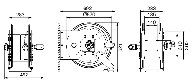
Series 617, inlet 1 1/2"
