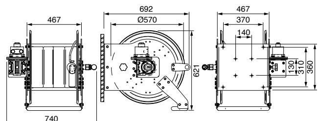
Series 638, inlet 1"
