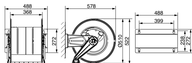
Series 560
