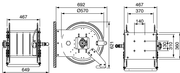
Series 637, inlet 1"
