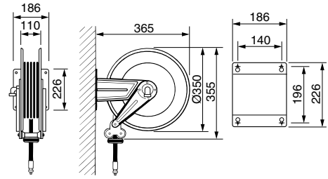
Series 300
