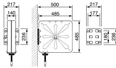
Series 440
