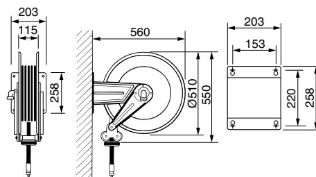
Series 530
