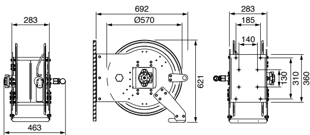
Series 617, inlet 1"
