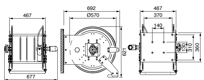
Series 637, inlet 1 1/2"
