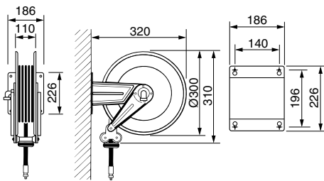
Series 270
