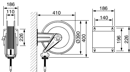
Series 350
